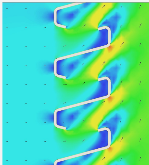
EFD simulation
