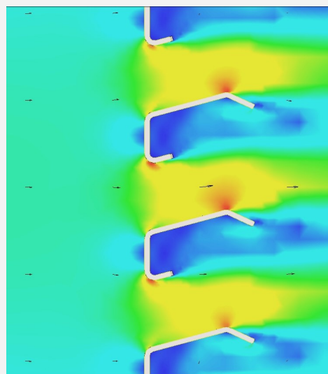
EFD simulation
